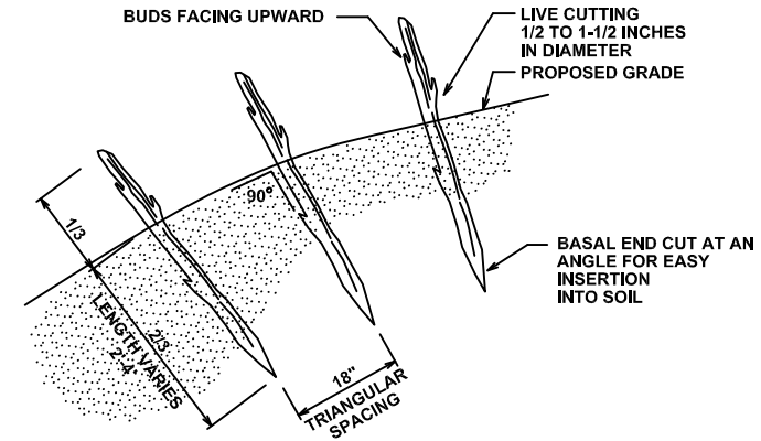
LIVE STAKE INSTALLATION CROSS SECTION-TYPICAL
