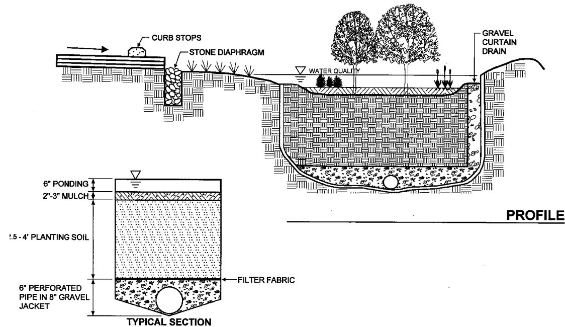
TYPICAL SECTION
