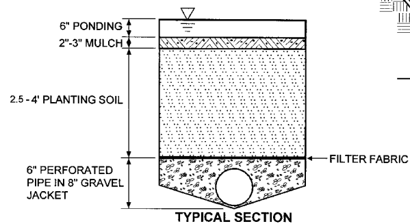
TYPICAL SECTION
