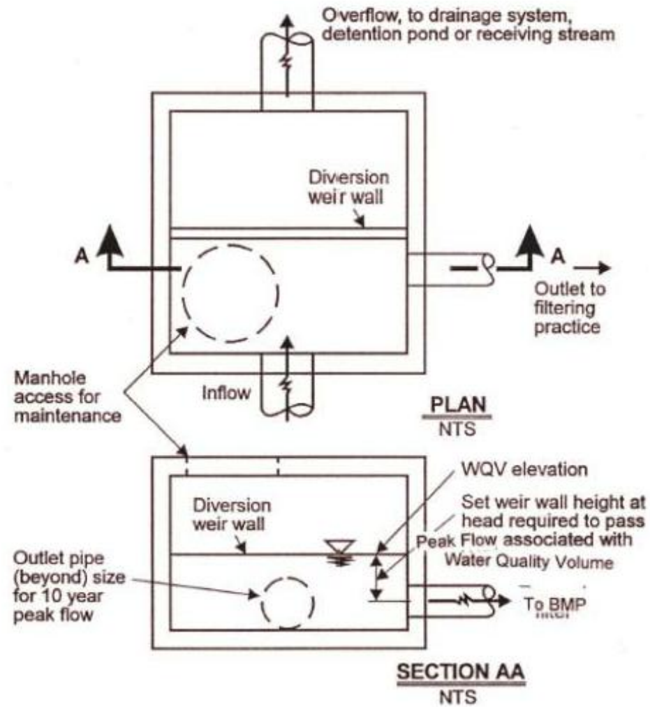
FLOW SPITTER PLAN AND PROFILE VIEWS - TYPICAL
