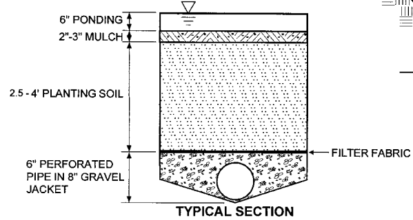
TYPICAL SECTION
