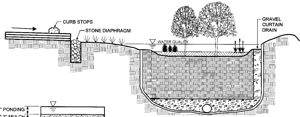
PROFILE
