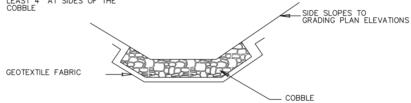
TYPICAL SECTION COBBLE WEIR
