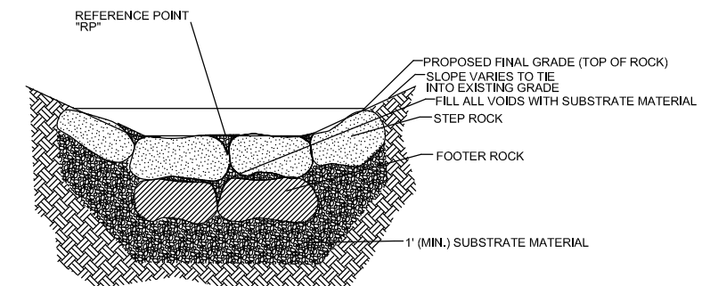
STEP POOL - STEP CROSS SECTION - TYPICAL
