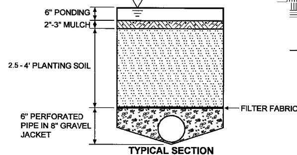
TYPICAL SECTION
